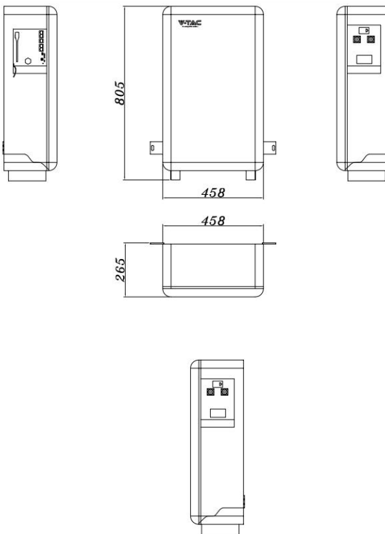
Fig. 5-1 Product Dimensions
